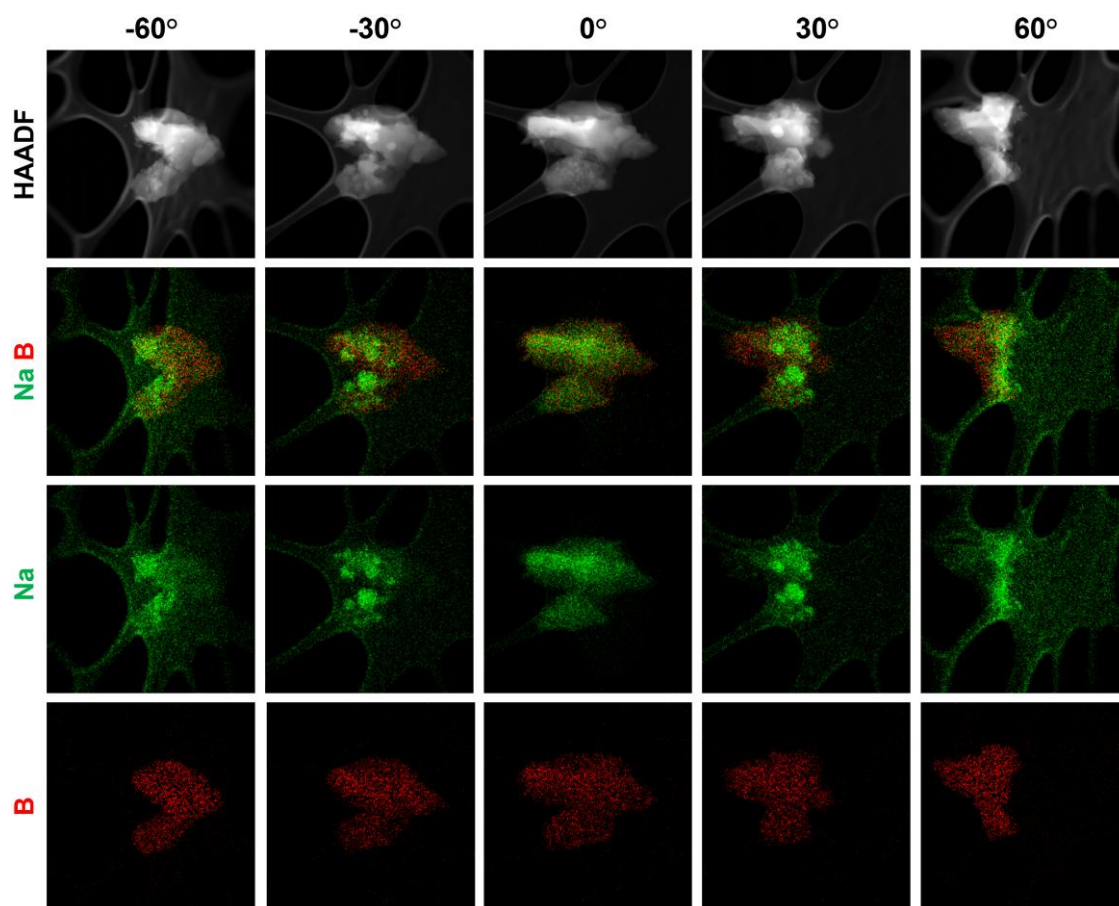
Fig. 3 . STEM + XEDS tomography sequence of NBH particle. Separate views of HAADF signal and integrated net signal spectra for sodium + boron, sodium, and then boron are shown every 30°. The middle column was acquired first in the acquisition scheme.
