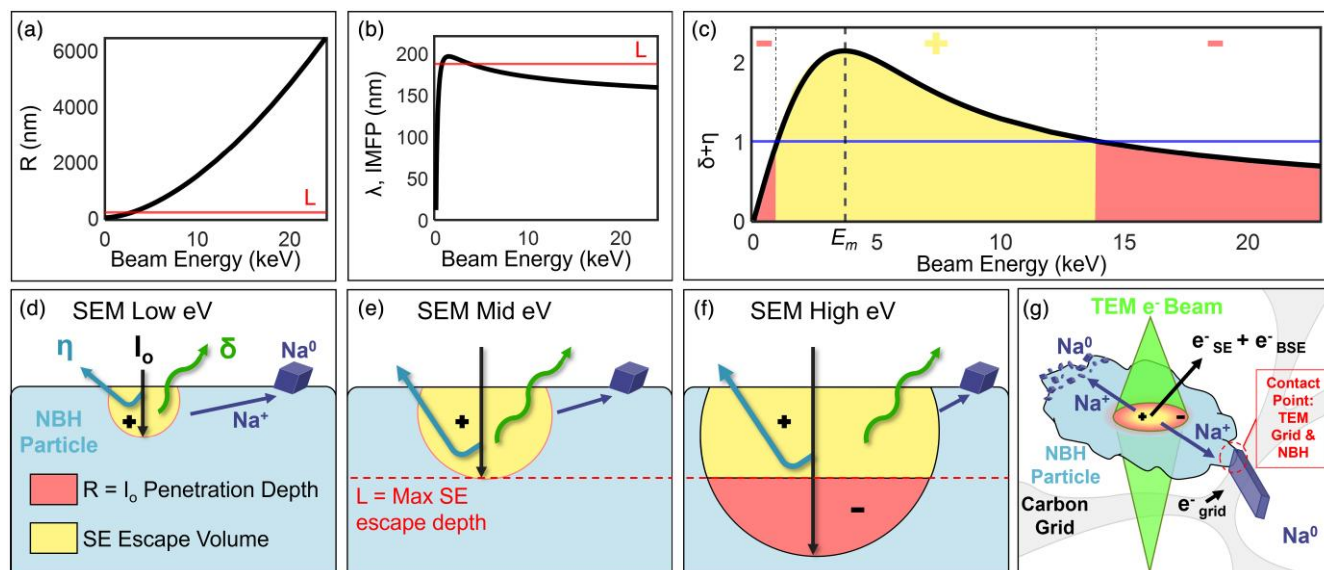
Fig. 7. Calculations for electron yield curve and the resulting schematic models of electron beam interaction with NBH. (a) R as a function of incident beam energy into NBH. (b) Inelastic mean free path of electrons through NBH as a function of electron beam energy. (c) Approximated standard yield curve for NBH as a function of beam energy. (d) Schematic for low I_0 . (e) Case for R \approx SE escape volume. (f) Case for R \gg SE escape volume. (g) Schematic for TEM electron bias of a thin sample at high keV and the resulting motion of electrons and sodium ions through the sample.
