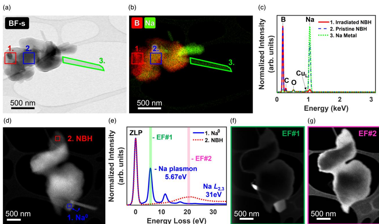
Fig. 2. Spectroscopic studies of NBH electron irradiation damage. (a) Bright-field STEM image of the NBH particle on the lacey carbon TEM grid with green, blue, and red overlays of selected areas integrated into XEDS spectra displayed in (c). Data collected at room temperature, 300 keV, 100 pA, and 1 ms/pixel. The left area was exposed to the electron beam for TEM study and recorded reduced sodium K-shell signal intensity. The center region of the particle is comprised of bulk NBH. The right side features sodium crystals grown from the contact point of the NBH particle and the carbon TEM grid. (b) Boron and sodium XEDS hyperspectral image (HSI) of the NBH particle and sodium crystal growths. HSI is comprised of the net signal of six integrated frames. (c) Extracted spectra from the selected areas in (a). (d) HAADF STEM micrograph pre-EELS hyperspectral image acquisition with two sodium crystals grown. (e) Two low-loss energy spectra from the hyperspectral image integrating 1000 frames: blue, lower corner, metallic plasmon signature matching the literature values for sodium metal, with the primary peak at approximately 5.67 eV. Faint sodium L_{2,3} at 31 eV. Red, no metallic plasmon signature, with an initial low-loss peak near 20.7 eV. Energy-filtered (EF) images for the (f) sodium plasmon and (g) NBH low-loss peak were extracted from the spectrum image and clearly segment the sodium crystal from the SSE particle.
