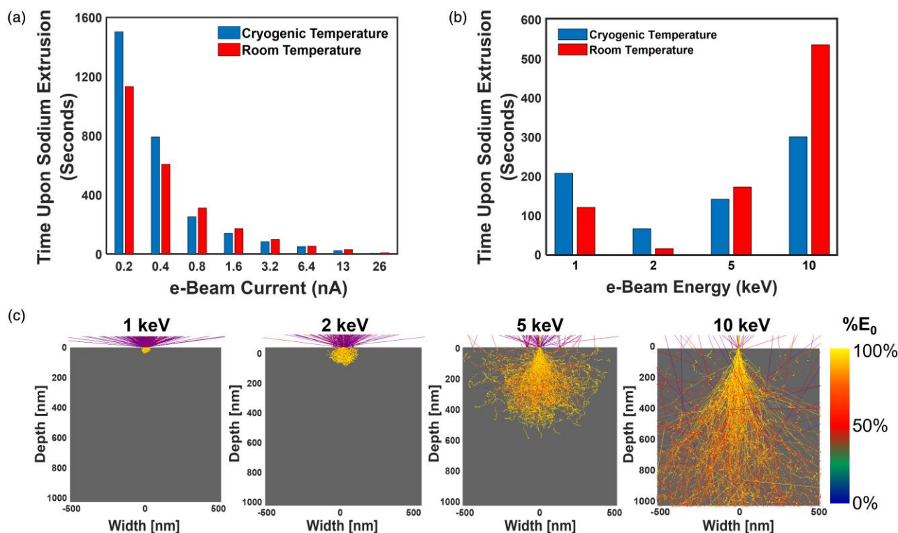
Fig. 6. Time until damage matrix for SEM dose experiments and simulated yield from Monte Carlo mirrors of the evaluated SEM beam energies. (a) SEM dose experiment matrix comparing the time until sodium extrudes from the surface of the NBH at varied beam currents and temperatures. (b) Similar SEM dose experiment matrix evaluating the effect of e-beam energy and temperature. (c) Displays electron dispersion for 1, 2, 5, and 10 keV CASINO Monte Carlo simulations of a 5 \mu\text{m}^3 volume (magnified to 1 \mu\text{m}^3 ) of NBH.
