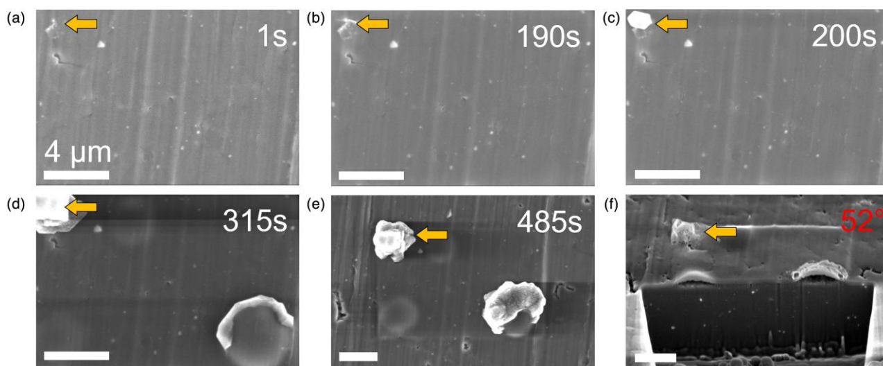
Fig. 5. Inert transfer cryo-SEM damage experiment of a mixed-anion NBH pellet at 5 kV, 1.6 nA, and 500 ns pixel -1 with a field of view of approximately 12 \mu\text{m} \times 17 \mu\text{m} (see Supplementary Supplementary Video 3 ). (a,b) The sample appeared unchanged for 190 s. (c) At 200 s, a faceted sodium crystal extruded and grew from the surface. (d) Surface perturbances became apparent and then burst after 300 s. (e) After approximately 500 s, we demagnify to reveal that the electron beam-dosed region has swollen. Several perturbances have grown on the surface. (f) Next, cross sections of the dosed area were revealed with a Ga + ion beam at 30 kV and 2.7 nA (see Supplementary Supplementary Video 4 ). All scale bars are 4 \mu\text{m} .
