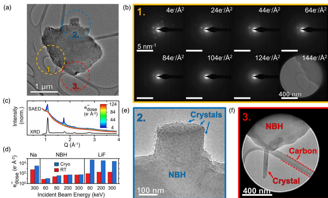
Fig. 1. Low-electron-dose-resolved TEM and SAED experiment for NBH irradiation damage. (a) Low-dose TEM image of crystalline \text{Na}_2(\text{B}_{10}\text{H}_{10})_{0.5}(\text{B}_{12}\text{H}_{12})_{0.5} particle. Three regions of sequentially staged experiments conducted on the same particle and described herein are circled. All three stages (a,b,c,e,f) were conducted at 300 keV, room temperature, 100 pA, and 1\ \mu\text{m} probe diameter for a d_{\text{rate}} of 8\ \text{e}^{-}\text{\AA}^{-2}\text{s}^{-1} . (b) Diffraction experiment sequence conducted as stage 1 (yellow circle). (c) Radial integrated diffraction profile from the SAED experiment (c) compared with capillary XRD acquired with Mo K alpha radiation. (d) SAED electron dose stability comparison of sodium metal, NBH, and LiF at room temperature and cryogenic liquid nitrogen temperature across a range of energies. (e) Stage 2 (blue circle) small crystal nuclei on opposing sides of the NBH particle from the diffraction experiment site. (f) Stage 3 (red circle) large crystal nucleation at the contact point between NBH and lacey carbon TEM grid.
