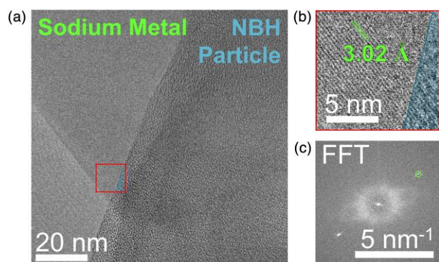
Fig. 4 . HREM of sodium and NBH interface. (a) Drift-correlated frame-integrated image at the NBH particle | sodium metal interface, recorded every 0.5 s at d_{\text{rate}} of 20 \text{ e}^- \text{Å}^{-2} \text{s}^{-1} for 2.5 s for d_{\text{total}} of 100 \text{ e}^- \text{Å}^{-2} . Pixel size is 49.55 pm. (b) Digitally magnified interface. (c) The FFT of the micrograph.
