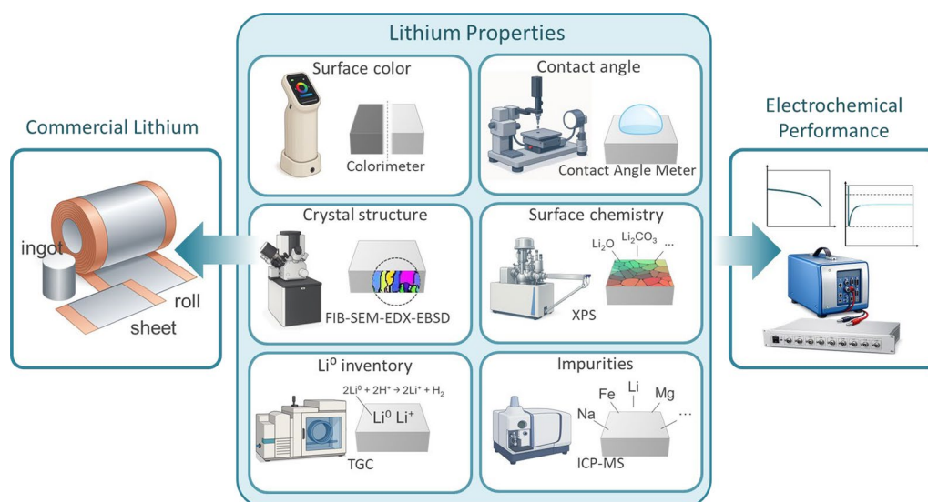
Fig. 1 Characterization workflow using integrated metrology tools for comprehensive analysis of lithium metal foil prior to its application in LMBs
