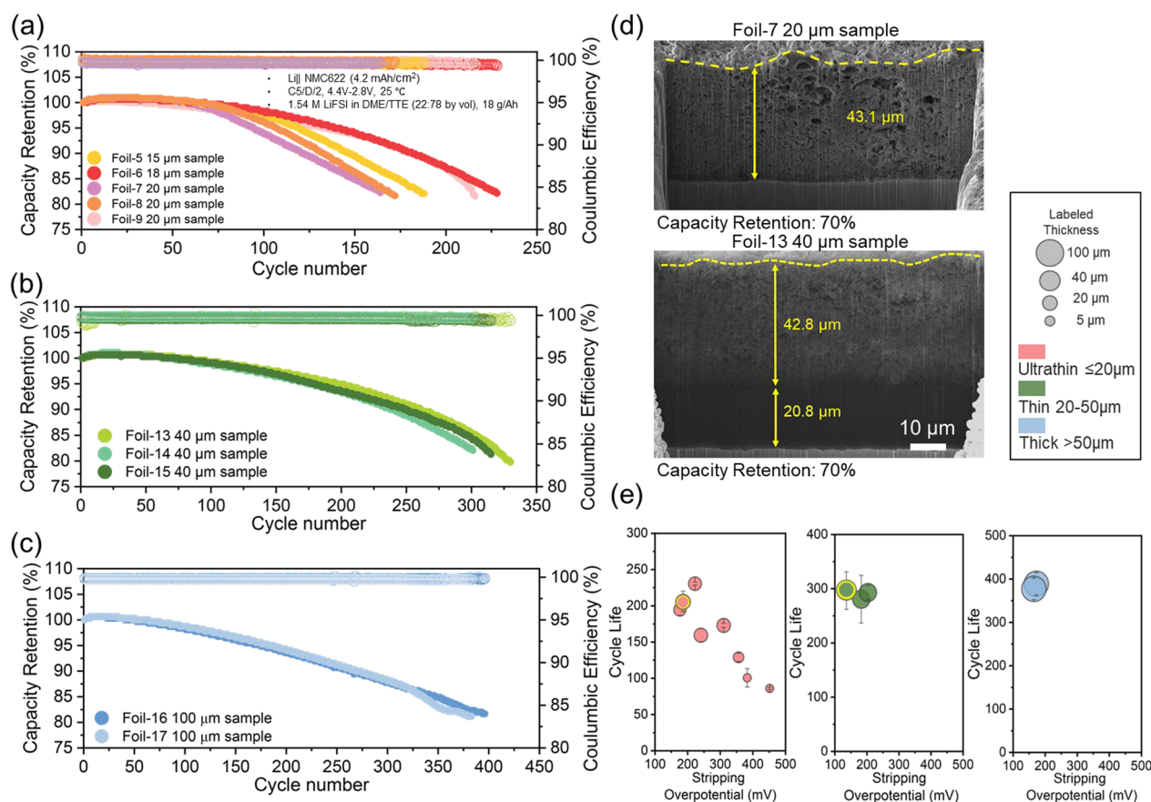
Fig. 5 Capacity retention over cycles in Li||NMC622 full cells using a ultrathin lithium foils, b thin lithium foils, and c thick lithium foils. d PFIB-SEM cross-section images of LMAs after reaching 70% capacity retention with different initial lithium thickness. e Cycle life of lithium foils in Li||NMC622 full cells as a function of stripping overpotential in Li||Cu cells
