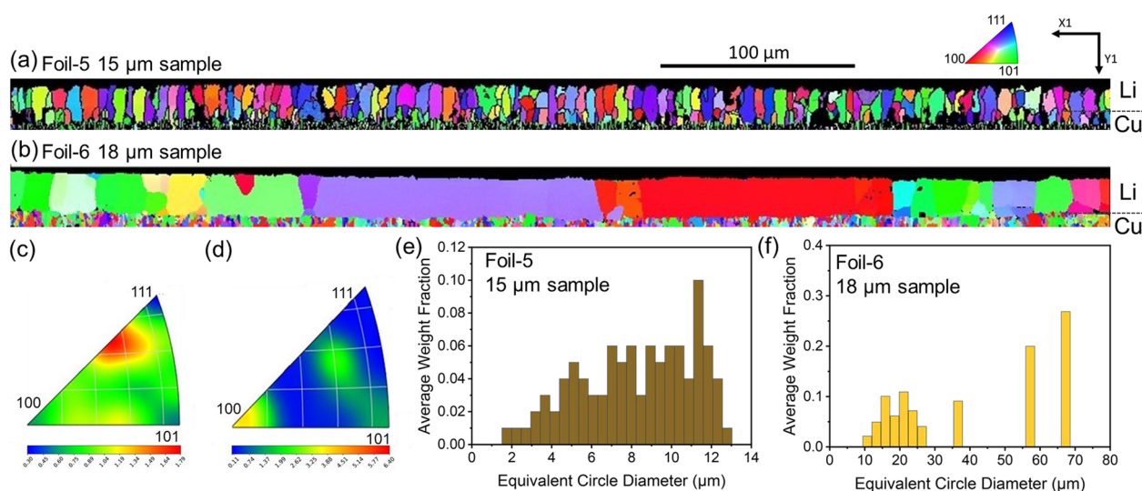
Fig. 6 EBSD mapping results along the growth direction, the inverse pole figures, and grain size analysis of a, c, e Foil-5 15 \mu\text{m} sample and b, d, f Foil-6 18 \mu\text{m} sample
