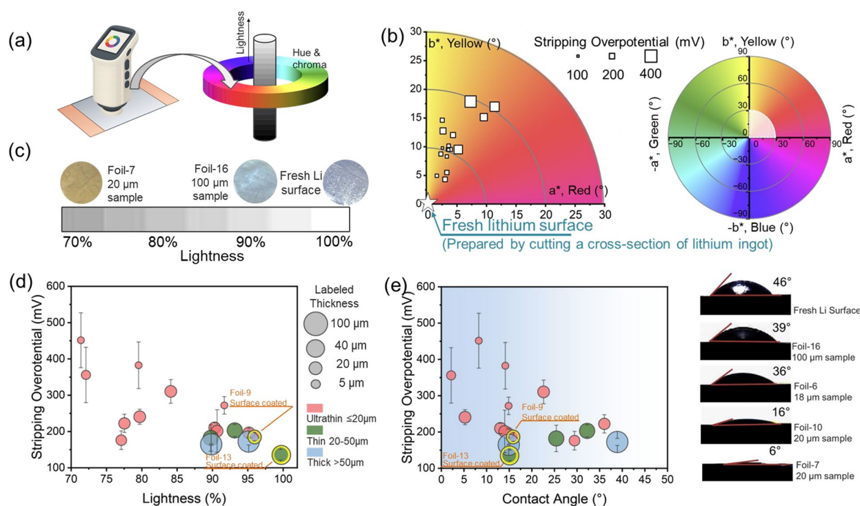
Fig. 3 a Schematic illustration of color space measurements of lithium metal using a colorimeter. b Hue and chroma map of lithium metal samples. The size of the sample spot represents the stripping overpotential of the sample in a Li || Cu cell. The full color map is shown on the right side, where the focused sector is marked in white. c Photographic comparison of selected lithium foils arranged by surface lightness. d Stripping overpotential in a Li || Cu cell as a function of Li foil surface lightness. e Surface contact angle of localized high-concentration electrolyte (LHCE, 1.54 M LiFSI in DME:TTE = 22/78 v/v%) on lithium metal foil. Correlation between LHCE contact angle and stripping overpotential in a Li || Cu cell
