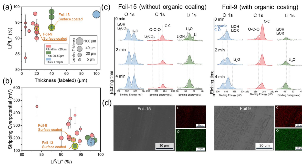
Fig. 4 a Lithium foil labeled thickness as a function of lithium purity. b Lithium purity as a function of stripping overpotential in \text{Li}||\text{Cu} cells. c XPS spectra of Foil-15 40 \mu\text{m} sample and Foil-9 20 \mu\text{m} sample. d Surface morphology and elemental mapping via SEM-EDX for Foil-15 40 \mu\text{m} sample and Foil-9 20 \mu\text{m} sample
