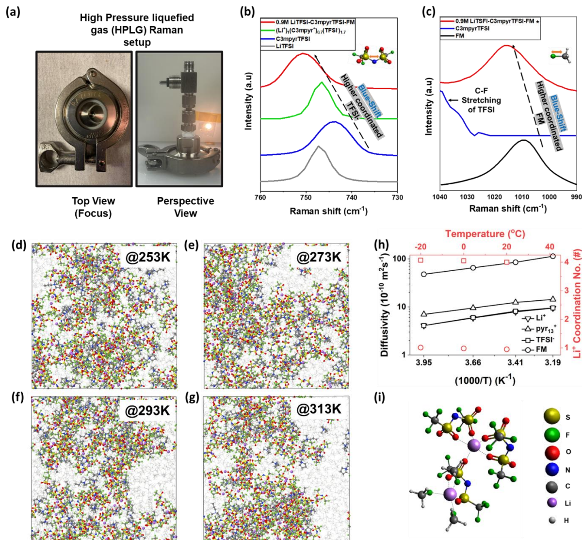
Fig. 3. (a) Top and perspective view of HPLG Raman setup. Raman spectra analysis of IL-LGE, LiTFSI, c3mpyrTFSI and FM probing (b) S-N-S bending mode of TFSI (c) C-F stretching mode of FM. Representative snapshot of MD simulation box of IL-LGE at (d) 253 K (e) 273K (f) 293K (g) 313K. (h) Temperature dependence of diffusivity of electrolyte species and Li + coordination number. (i) Representative cluster of solvated species of Li + in IL-LGE.
