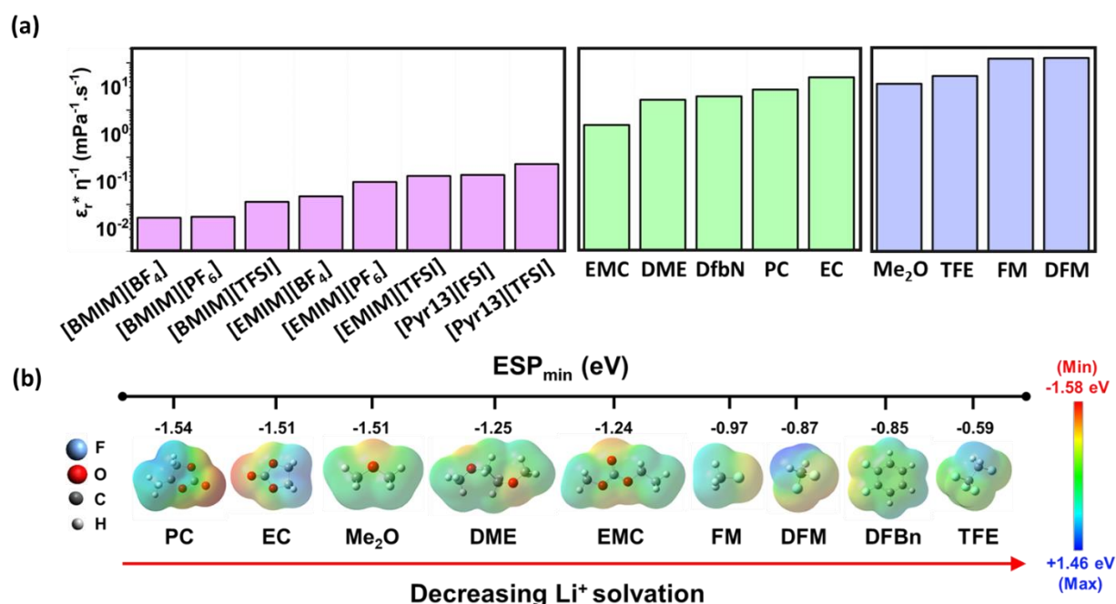
Fig. 1. Comparison of (a) dielectric-fluidity ( \epsilon_r^* \eta^{-1} ) factor values of ILs (pink), organic solvents (green), and liquefied gas solvents (blue) – calculated from literature [refs 13,18 - 24]. (b) ESP mapping minima and Li + solvating power screening of organic and liquefied gas solvents.
