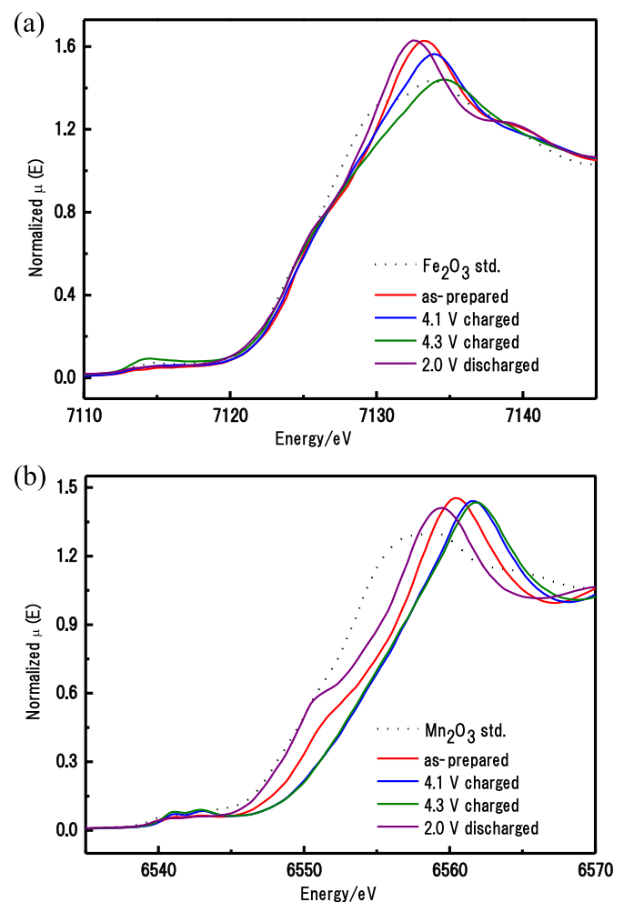
Fig. 3. (a) Fe K-edge and (b) Mn K-edge XAS analysis of \text{Na}_{2/3}\text{Fe}_{1/3}\text{Mn}_{2/3}\text{O}_2 charged to 4.3 V and discharged to 2.0 V.
