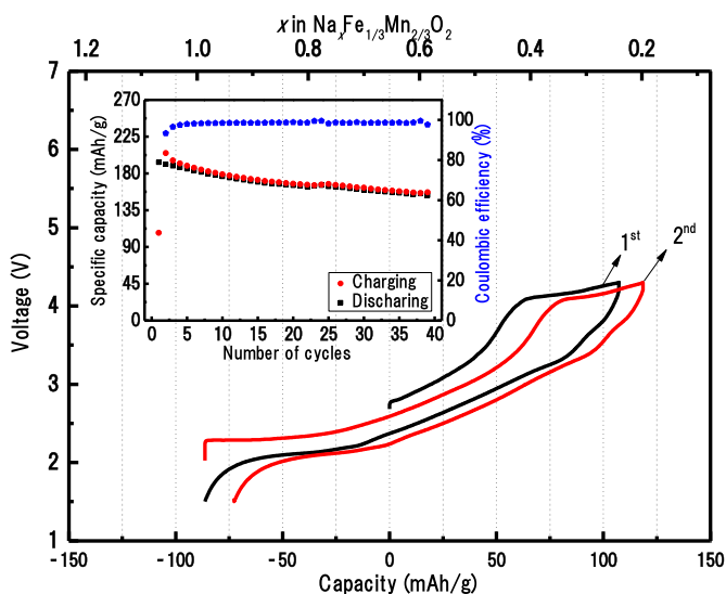
Fig. 2. Voltage profiles and the cyclability of \text{Na}_{2/3}\text{Fe}_{1/3}\text{Mn}_{2/3}\text{O}_2 at a rate of 12 mA/g in the voltage range of 1.5 V and 4.3 V.
