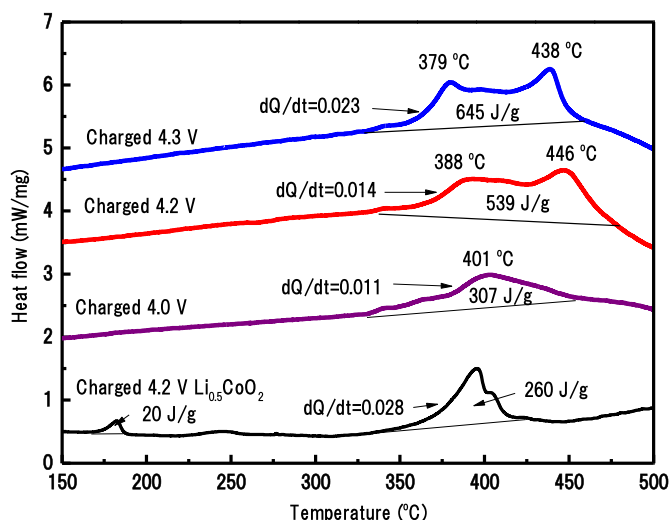
Fig. 4. DSC curves of \text{Na}_x\text{Fe}_{1/3}\text{Mn}_{2/3}\text{O}_2 charged to 4.0 V, 4.2 V, or 4.3 V, respectively. The samples were heated from room temperature to 500 °C at a rate of 5 °C/min.
