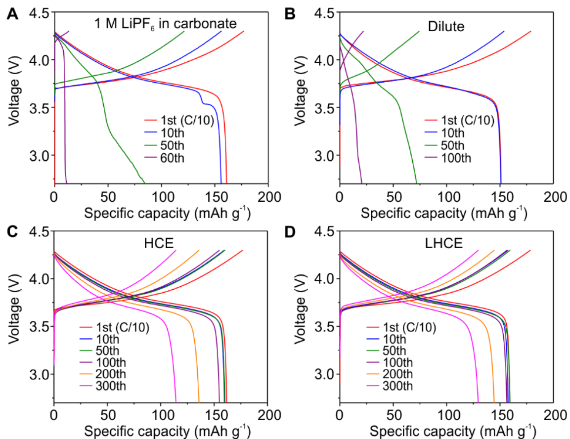
Figure S7. Voltage profiles of Li||NMC cells with 50 μm thick Li in different electrolytes: (A) 1 M LiPF 6 in EC/EMC (3:7 by vol.) with 2 wt% VC, (B) LiFSI-8TMS, (C) LiFSI-3TMS, (D) LiFSI-3TMS-3TTE.
