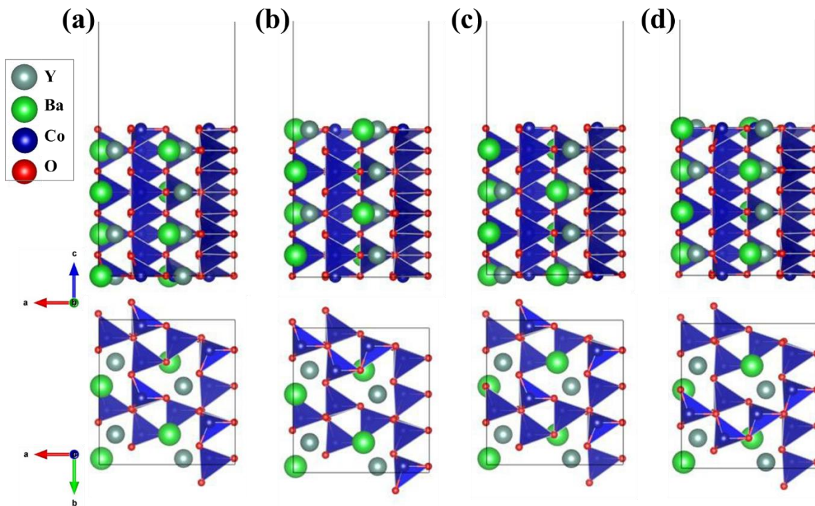
Figure 5.7 Possible terminations of YBaCo 4 O 7 (110)
