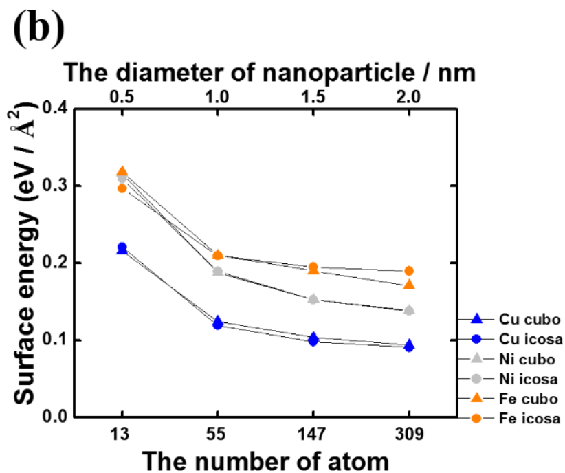
Figure 3.2 (a) Calculated conversion reaction voltage as a function of the size of M nanoparticle ( M = \text{Fe}, \text{Ni} and \text{Cu} ) formed. (b) Surface energy of M nanoparticle as a function of its size. The lower x-axis represents the number of atom contained in metal nanoparticle. The upper x-axis is the nanoparticle size in diameter which is approximate value. Detailed size information is demonstrated in Table 3.2
