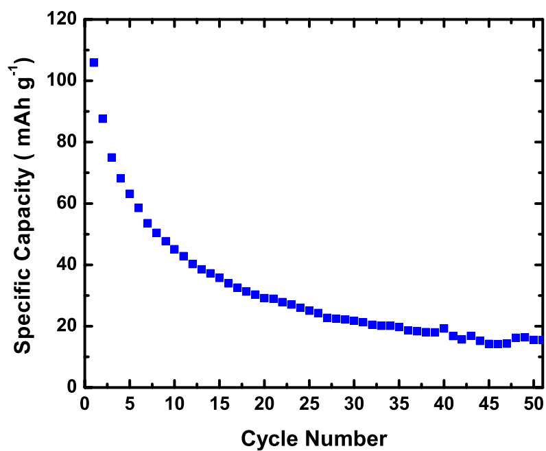
Figure 6.3 (a) Electrochemical charge and discharge voltage profiles between 2.80 and 4.95 V (vs. \text{Li/Li}^+ ); (b) Dependence of discharging capacity retention on number of cycles, the voltage range is 2.80 - 4.95 V (vs. \text{Li/Li}^+ ) at 0.1 \text{ C} = 167 \text{ mAh/g}
