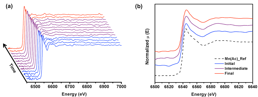
Figure 5.11 (a) Time evolution as a function of the reaction time for Mn K-edge XANES spectra during polyol process. (b) Selective XANES spectra of initial, intermediate and final stage including \text{Mn}(\text{CH}_3\text{COO})_2 dissolved in TTEG
