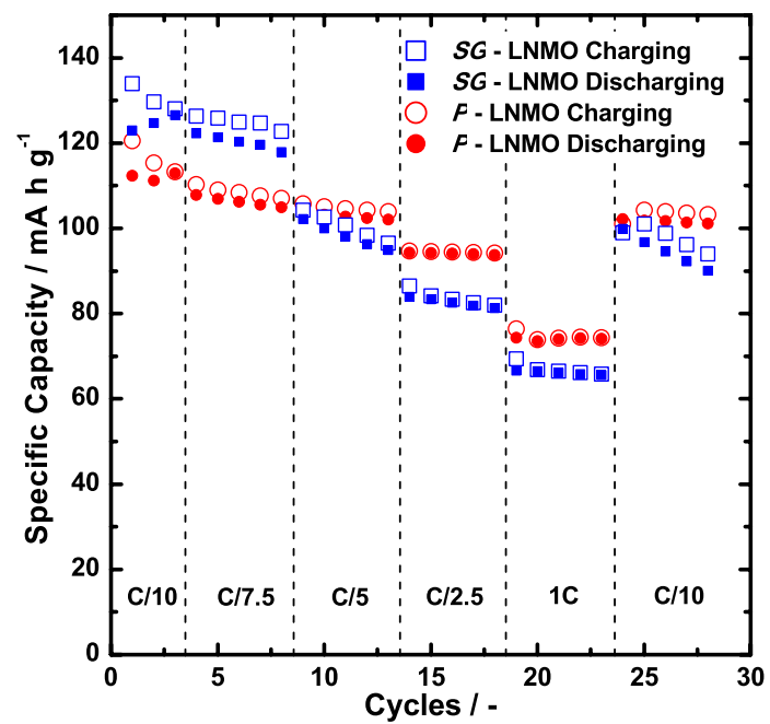
Figure 5.2 (c) Variation of capacity retention with various discharging rates obtained for \text{LiNi}_{0.5}\text{Mn}_{1.5}\text{O}_4 powders synthesized via sol-gel and polyol methods (continued)
