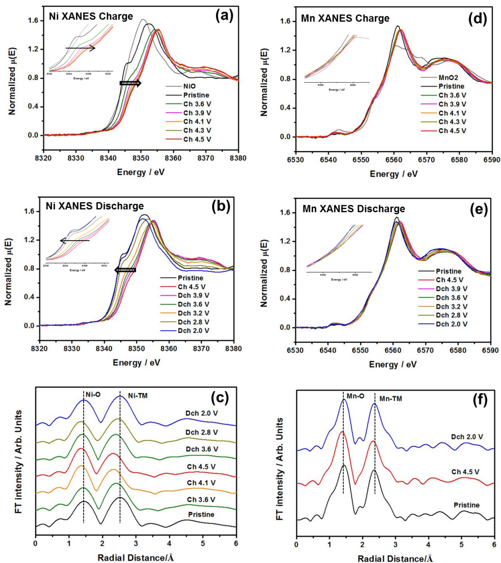
Figure 6.8. In-situ XAS analysis of \text{Na}_{0.78}\text{Ni}_{0.23}\text{Mn}_{0.69}\text{O}_2 electrodes at different SOCs during the first electrochemical cycle: (a) (b) XANES spectra at Ni K-edge, (d) (e) XANES spectra at Mn K-edge, and (c) (f) corresponding EXAFS spectra.
