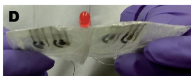
LED "OFF" ( 180^\circ Bend)
