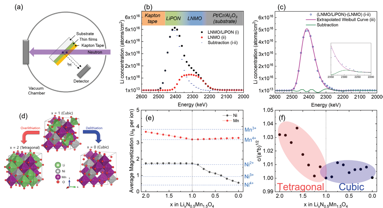
Figure 2. Li concentration across LNMO/LiPON interface. a) Schematic image of neutron depth profiling (NDP) setup. b) Li concentration profile (atoms cm -12 ) of LNMO/LiPON (black), bare LNMO (red), and subtraction of bare LNMO from LNMO/LiPON as a function of detected energy. c) Li concentration profile of subtraction of bare LNMO from LNMO/LiPON (blue, same data in (b)), Li concentration of bare LiPON simulated with Weibull function (magenta), and subtraction of simulated curve from (LNMO/LiPON-LNMO) curve (green). d) Structures of Li x Ni 0.5 Mn 1.5 O 4 , which are used for DFT calculation, at x = 1 (pristine), x = 0 (delithiated), and x = 2 (overlithiated). e) Averaged magnetization of Ni (black) and Mn (red) at each lithiated state of LNMO. f) Relative c length of the supercell at each lithiation state from x = 0 to x = 2 in L x NMO.
